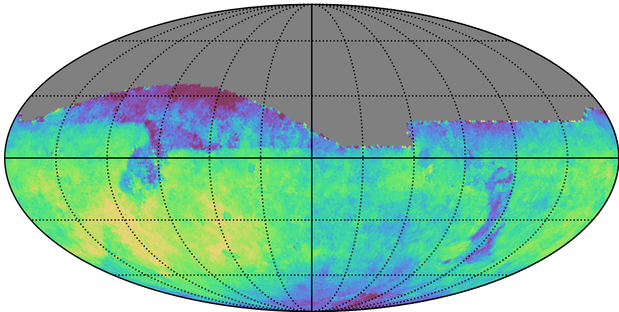
all_long_v3.4_10yrs All sky z band: Median saturation_mag
