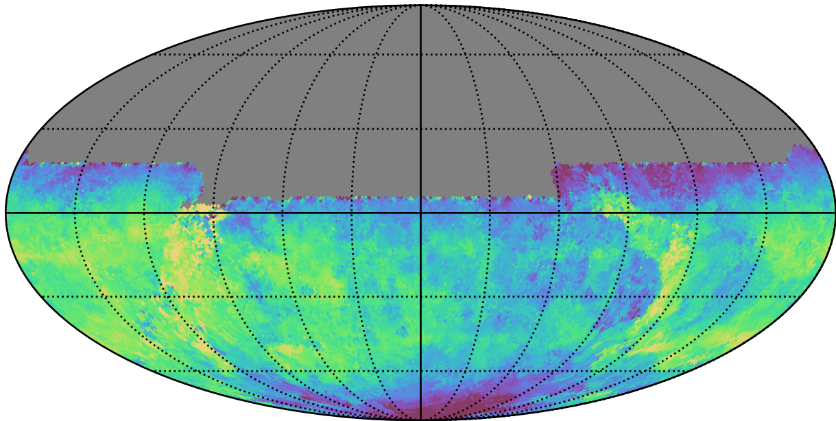
all_long_v3.4_10yrs All sky u band: Median saturation_mag
