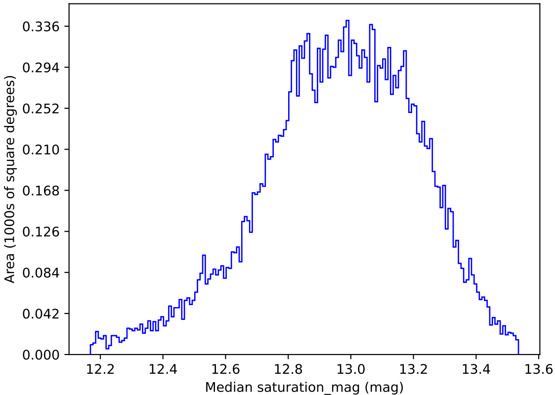
all_long_v3.4_10yrs All sky u band: Median saturation_mag
