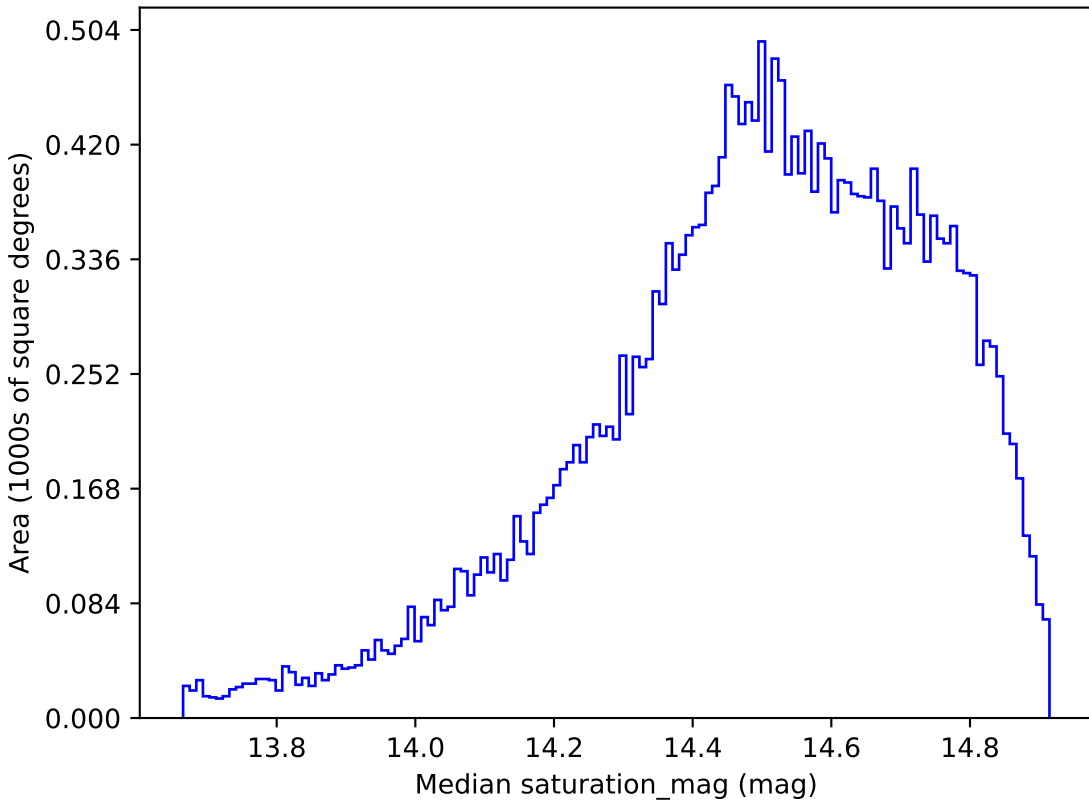
all_long_v3.4_10yrs All sky r band: Median saturation_mag
