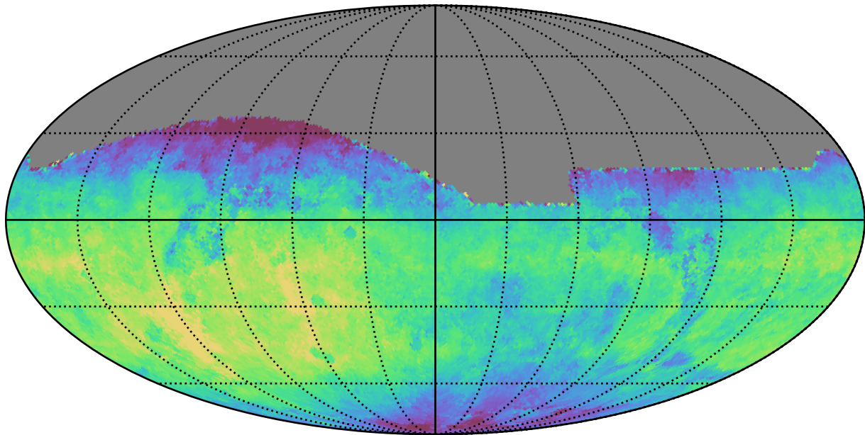
all_long_v3.4_10yrs All sky i band: Median saturation_mag
