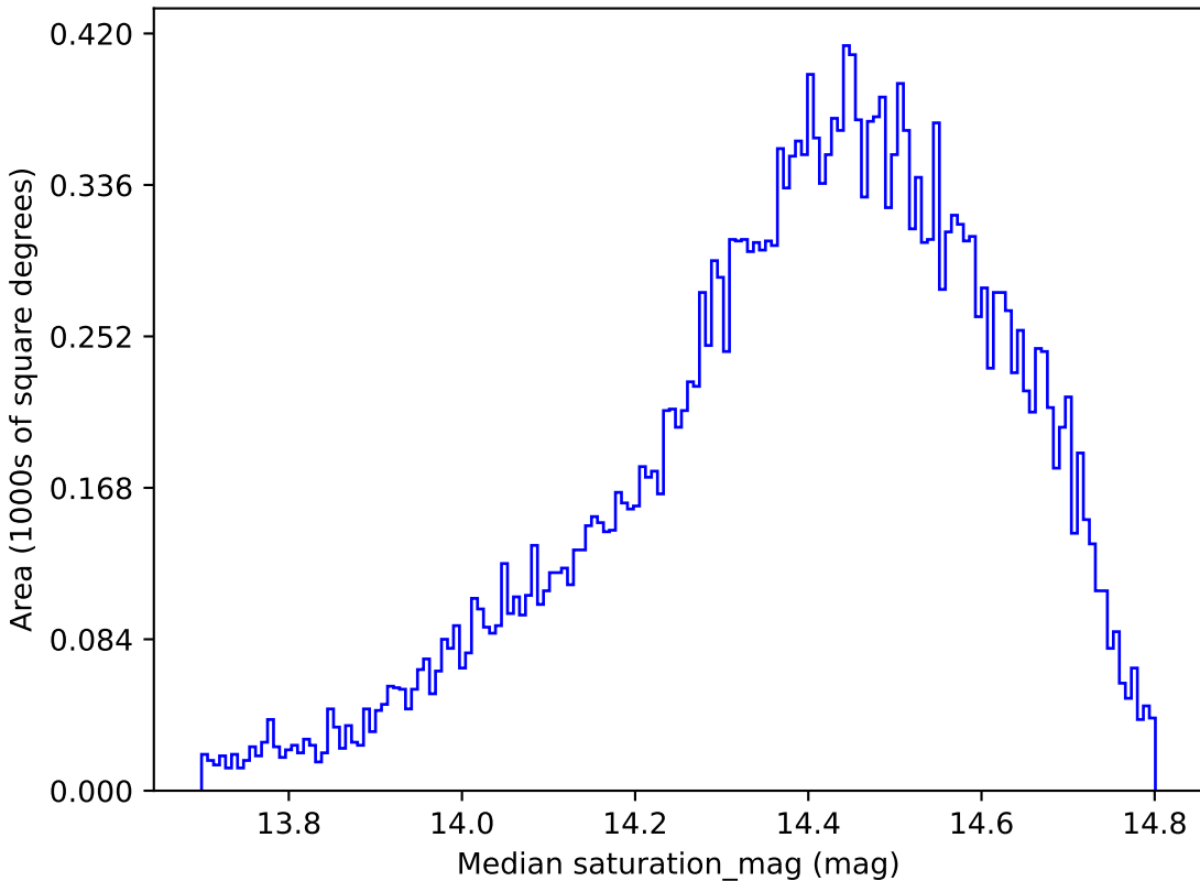
all_long_v3.4_10yrs All sky i band: Median saturation_mag
