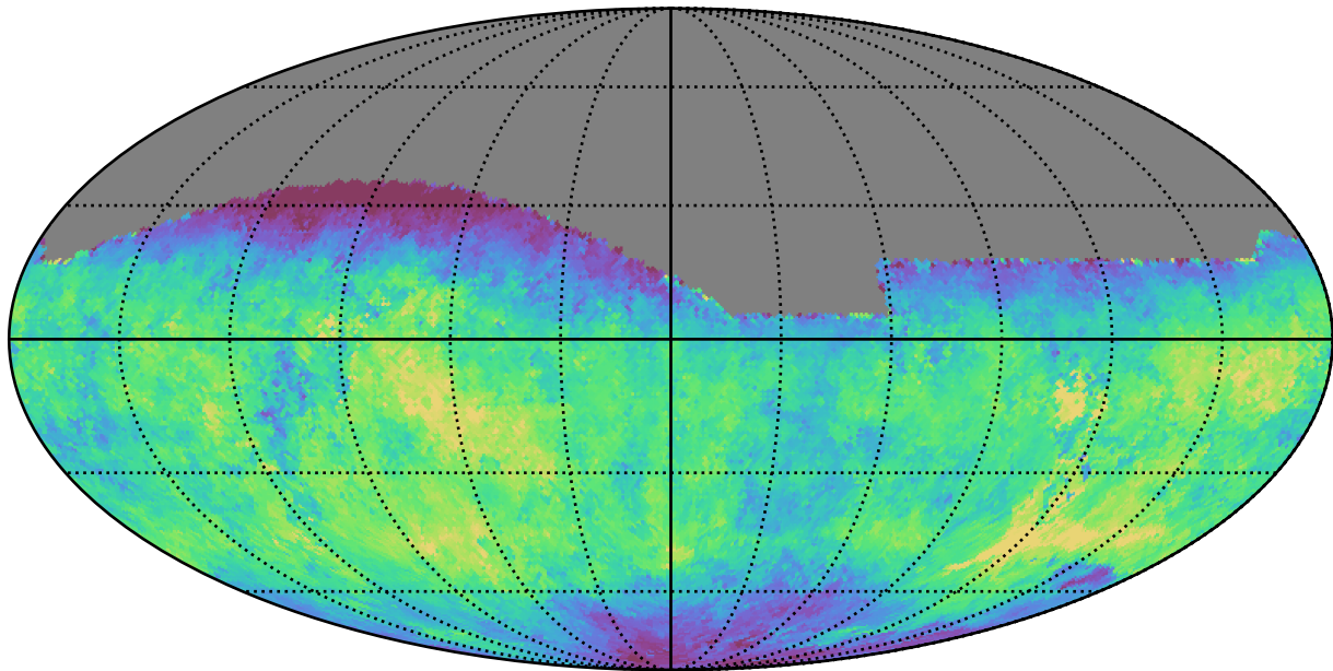
all_long_v3.4_10yrs All sky g band: Median saturation_mag
