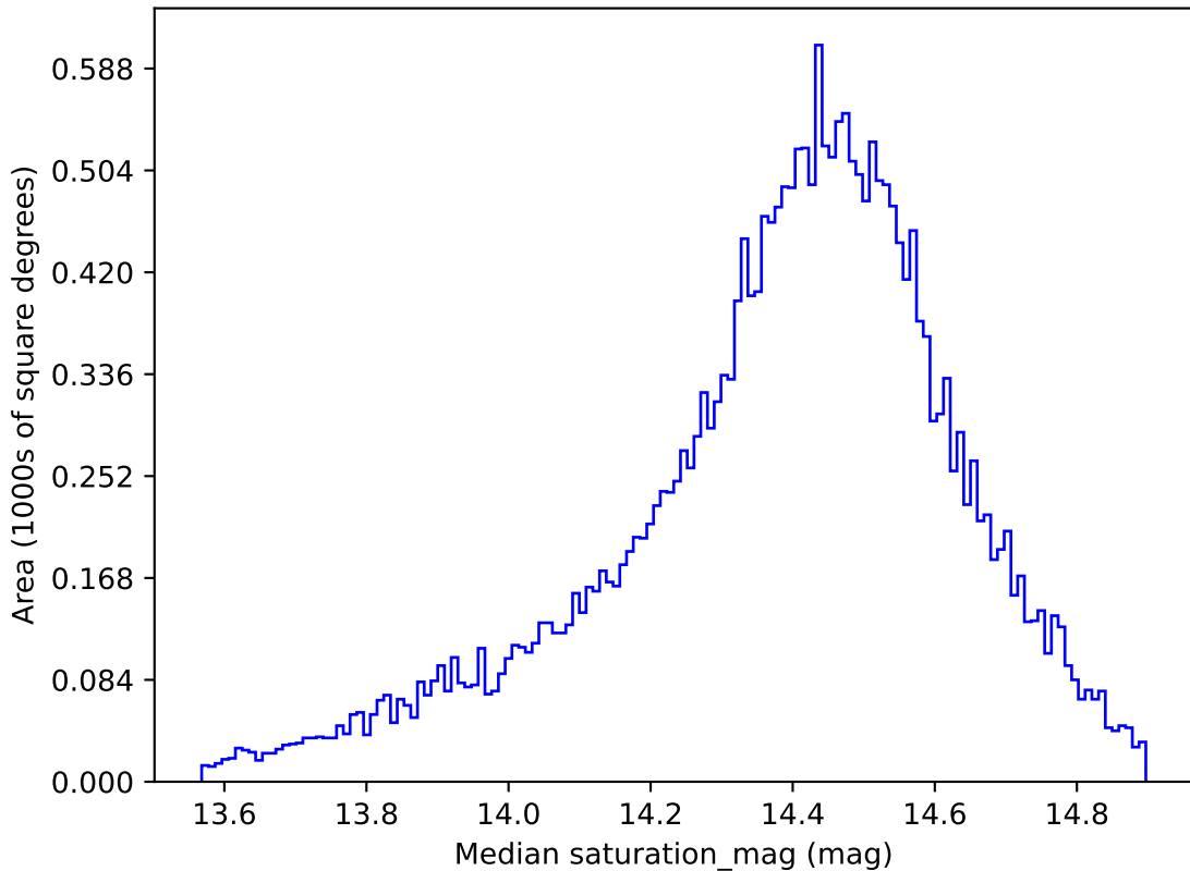
all_long_v3.4_10yrs All sky g band: Median saturation_mag
