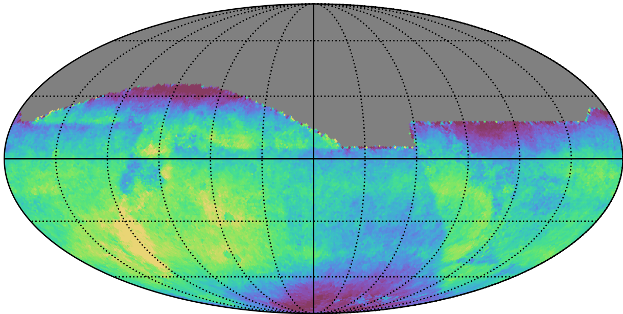
all_long_v3.4_10yrs All sky all bands: Median saturation_mag
