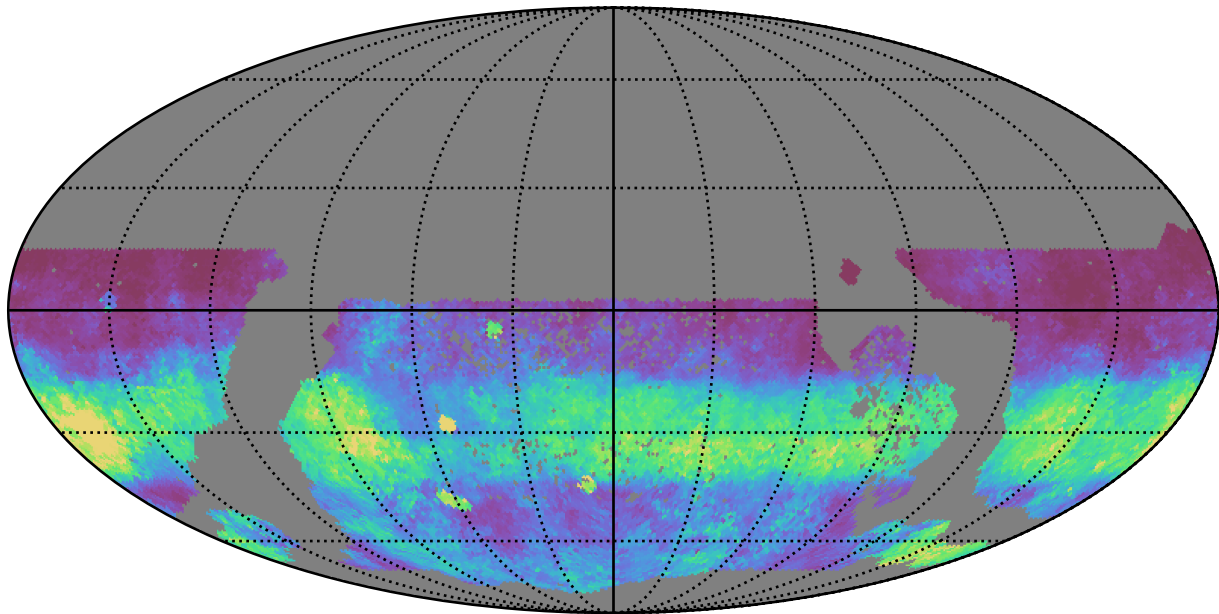
all_long_v3.4_10yrs WFD z band: Median normairmass
