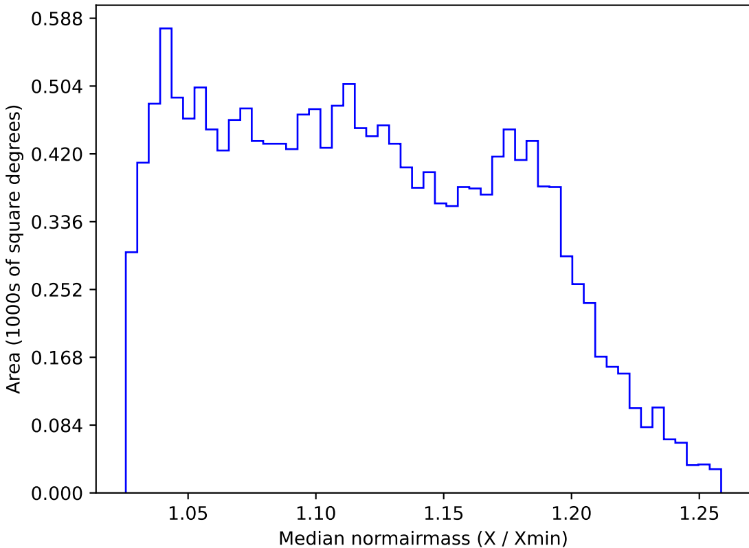
all_long_v3.4_10yrs WFD z band: Median normairmass
