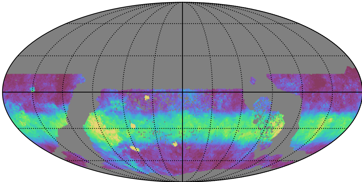
all_long_v3.4_10yrs WFD y band: Median normairmass
