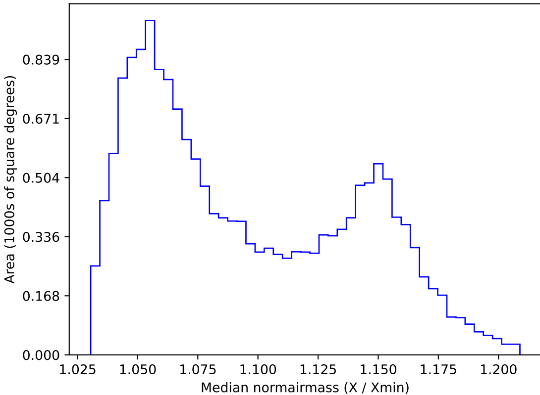
all_long_v3.4_10yrs WFD y band: Median normairmass
