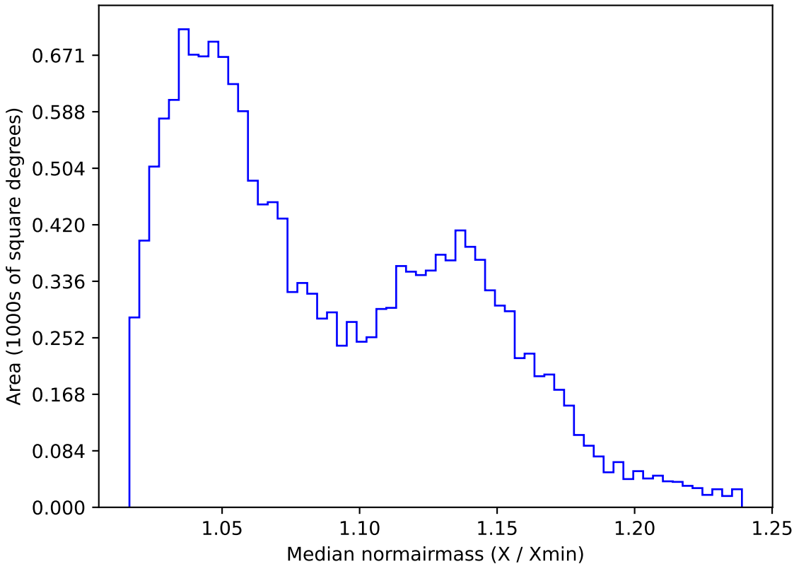
all_long_v3.4_10yrs WFD u band: Median normairmass
