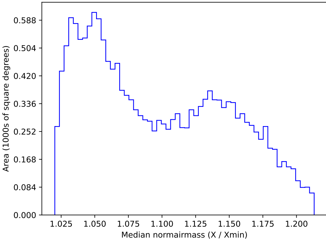
all_long_v3.4_10yrs WFD r band: Median normairmass
