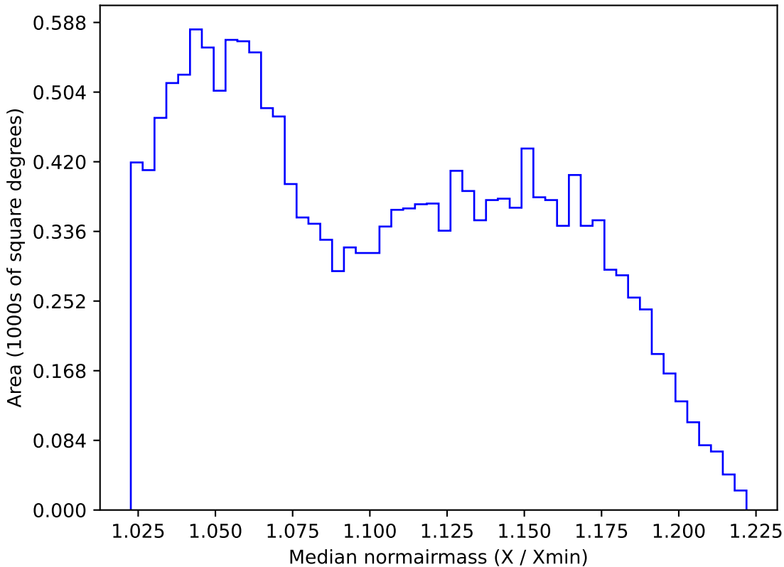
all_long_v3.4_10yrs WFD i band: Median normairmass
