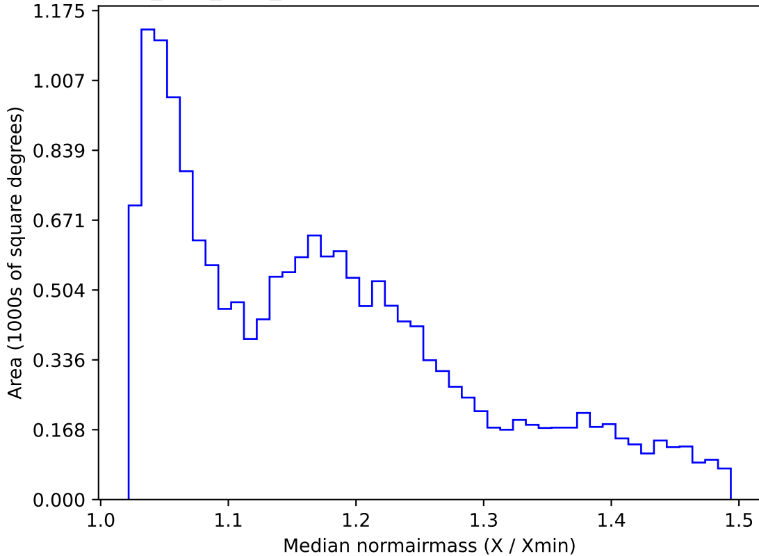
all_long_v3.4_10yrs WFD g band: Median normairmass
