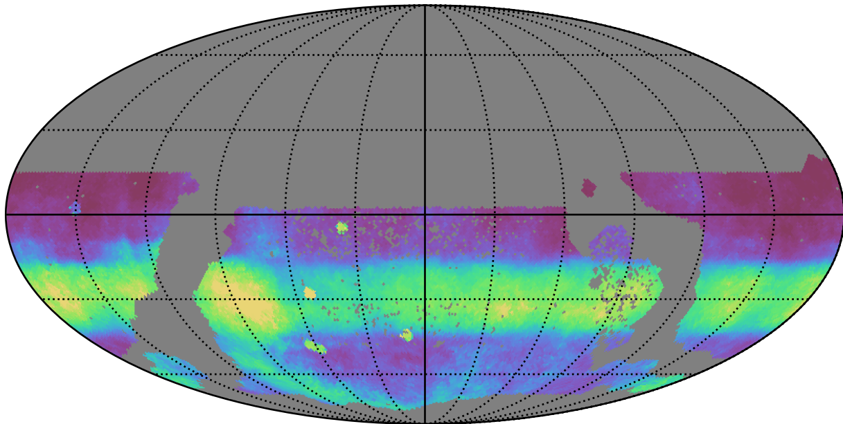
all_long_v3.4_10yrs WFD all bands: Median normairmass
