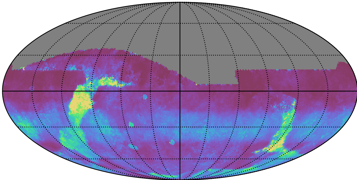
all_long_v3.4_10yrs All sky z band: Median normairmass
