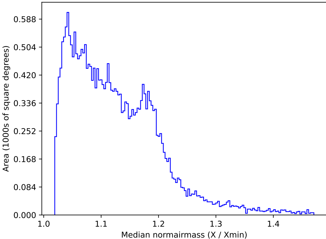
all_long_v3.4_10yrs All sky z band: Median normairmass
