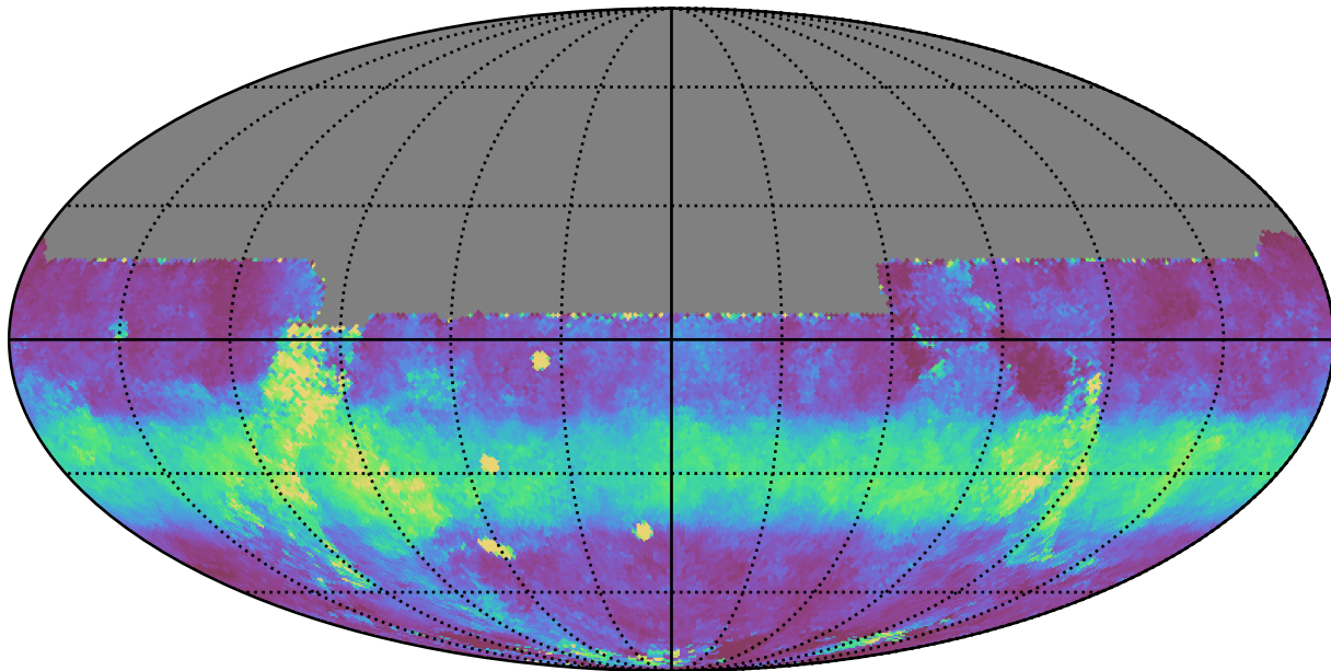
all_long_v3.4_10yrs All sky y band: Median normairmass
