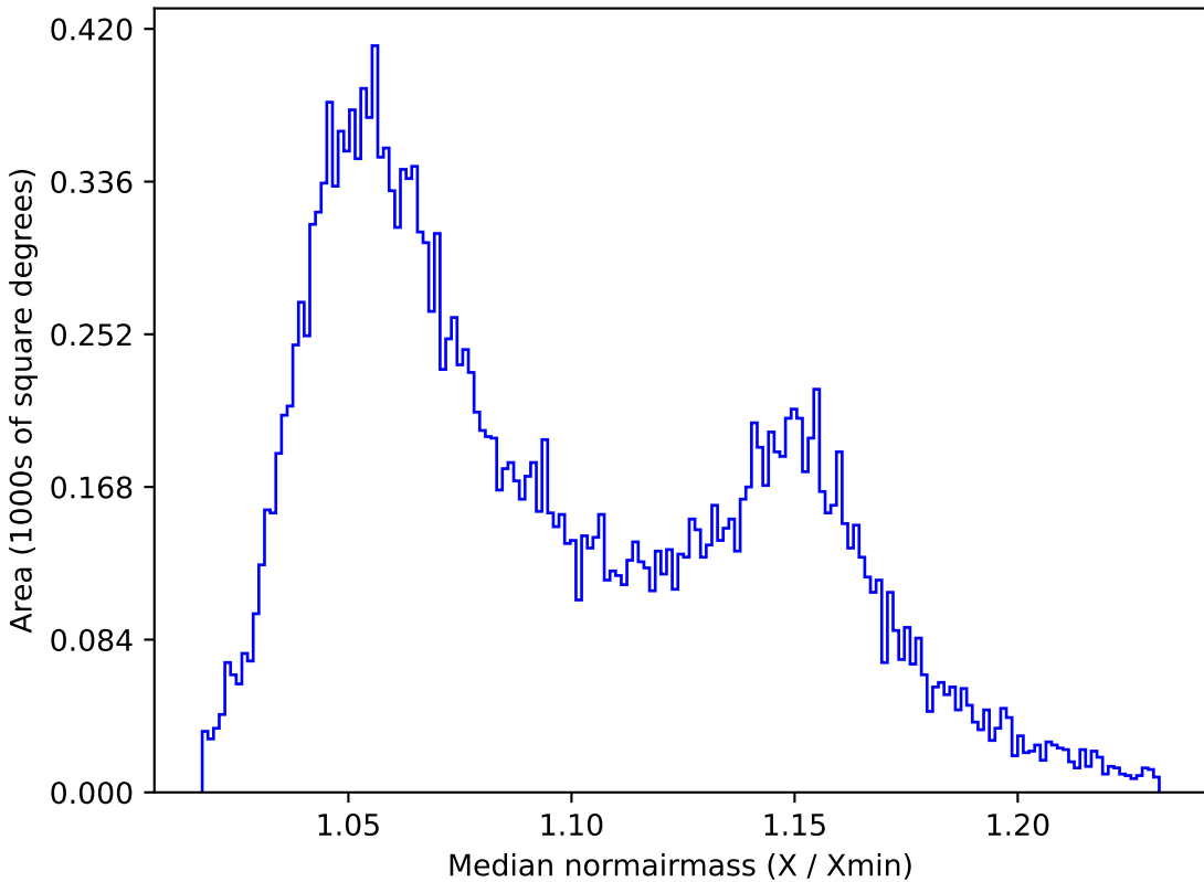
all_long_v3.4_10yrs All sky y band: Median normairmass
