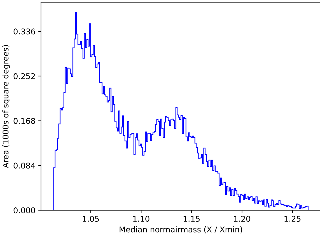
all_long_v3.4_10yrs All sky u band: Median normairmass
