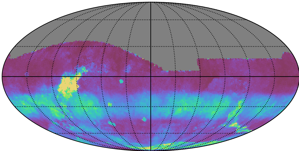
all_long_v3.4_10yrs All sky r band: Median normairmass
