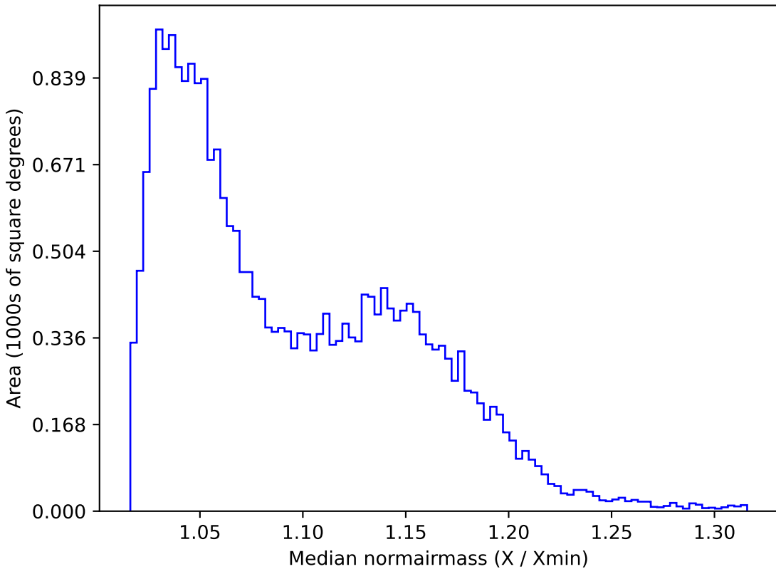
all_long_v3.4_10yrs All sky r band: Median normairmass
