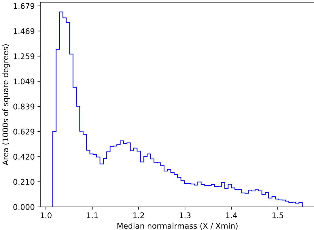
all_long_v3.4_10yrs All sky g band: Median normairmass
