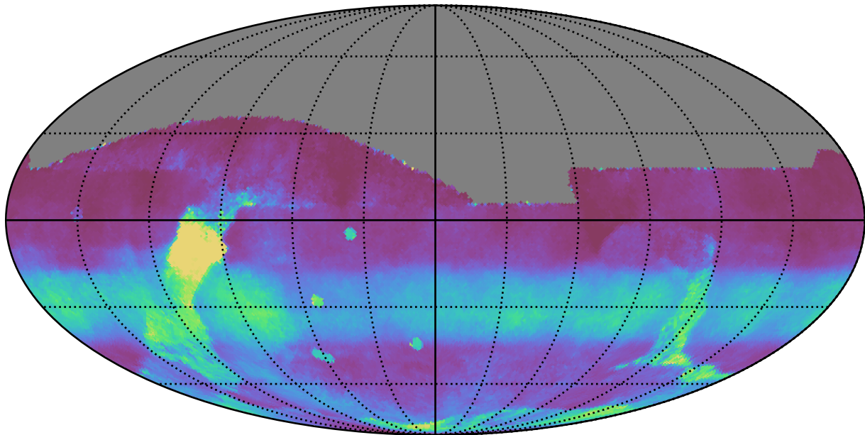
all_long_v3.4_10yrs All sky all bands: Median normairmass
