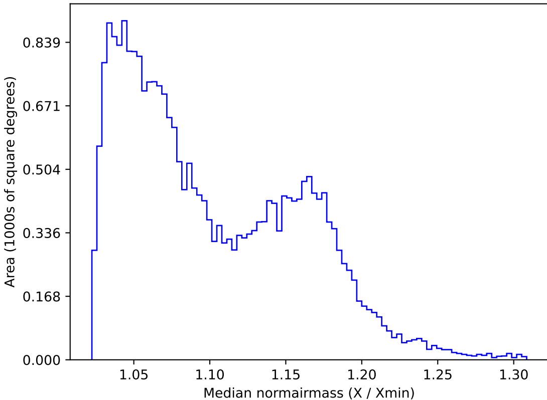
all_long_v3.4_10yrs All sky all bands: Median normairmass
