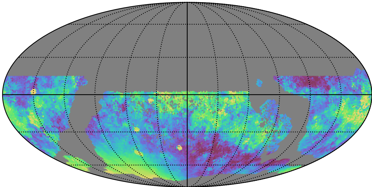
all_long_v3.4_10yrs WFD z band: Median moonDistance
