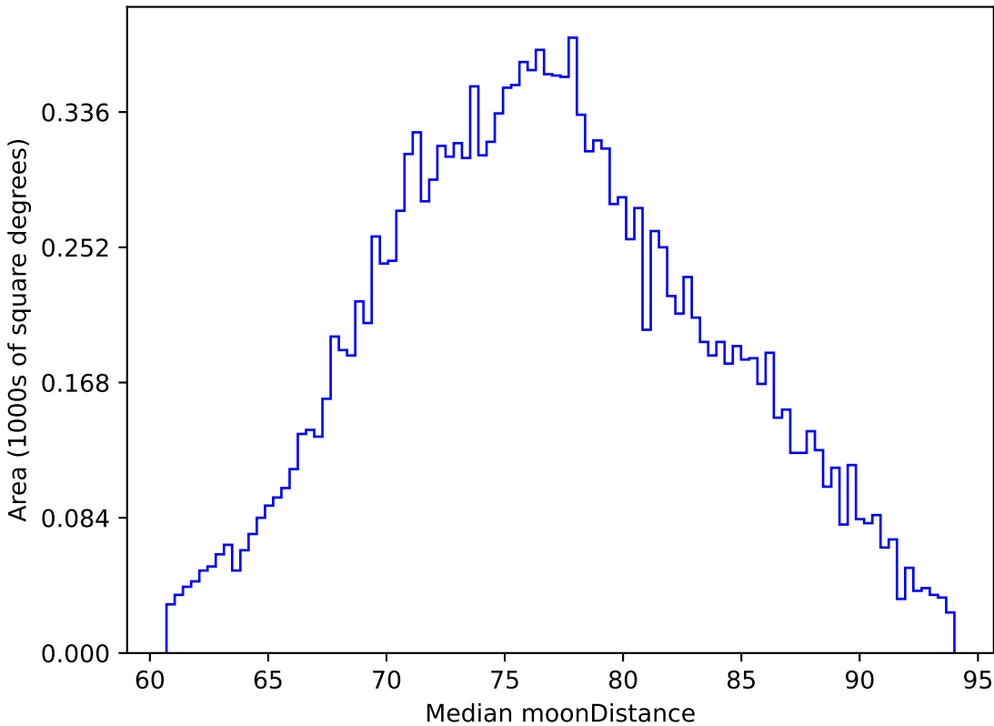
all_long_v3.4_10yrs WFD z band: Median moonDistance
