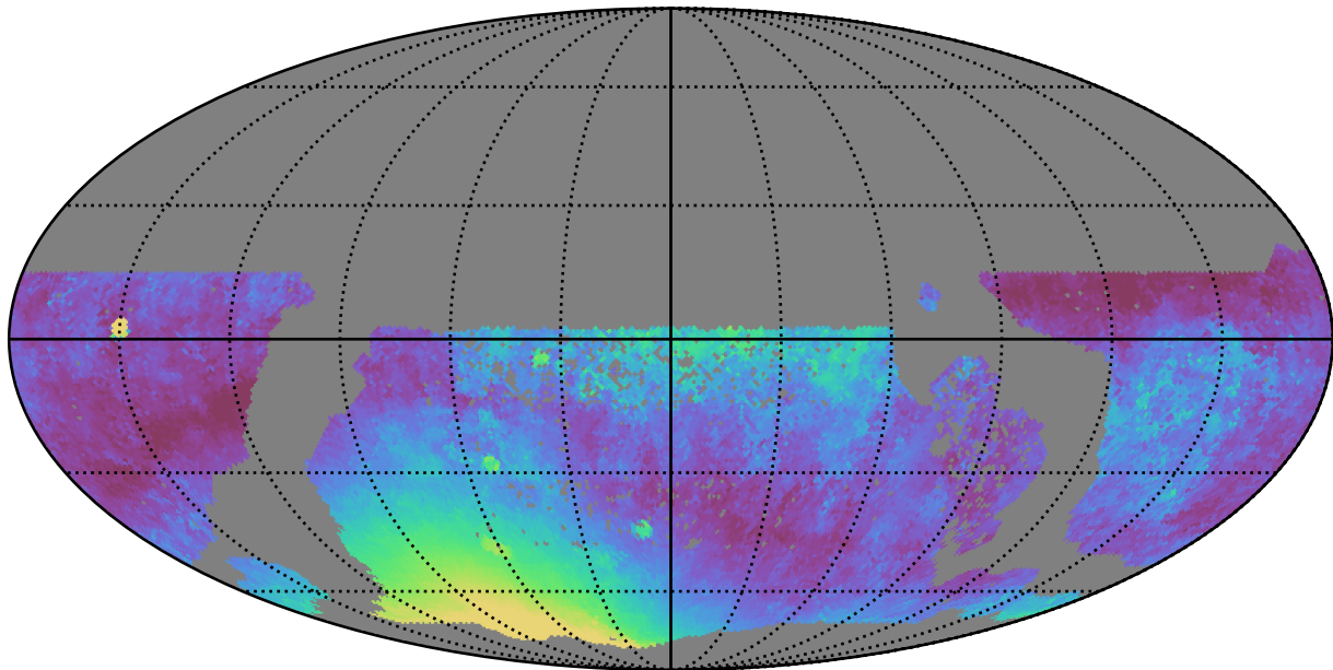
all_long_v3.4_10yrs WFD y band: Median moonDistance
