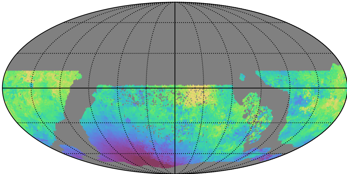
all_long_v3.4_10yrs WFD u band: Median moonDistance
