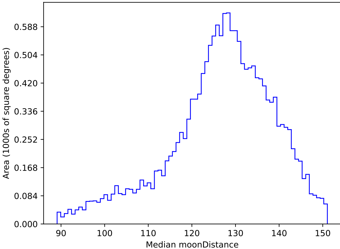
all_long_v3.4_10yrs WFD u band: Median moonDistance
