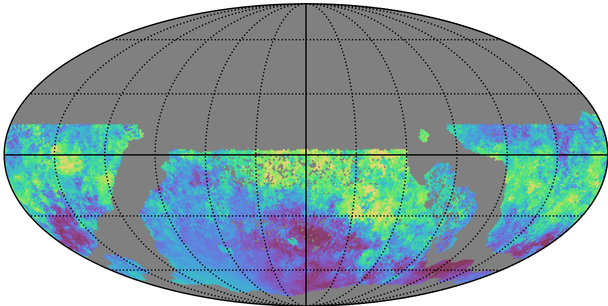
all_long_v3.4_10yrs WFD i band: Median moonDistance
