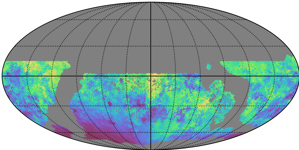
all_long_v3.4_10yrs WFD g band: Median moonDistance
