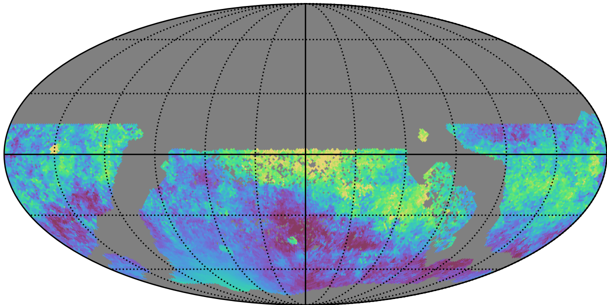
all_long_v3.4_10yrs WFD all bands: Median moonDistance
