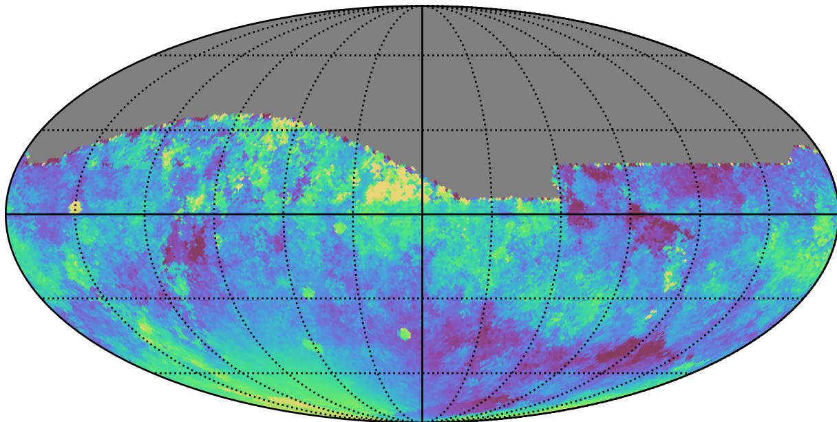
all_long_v3.4_10yrs All sky z band: Median moonDistance
