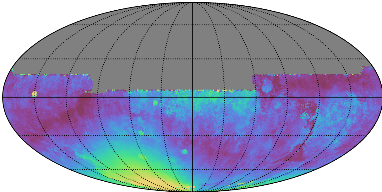
all_long_v3.4_10yrs All sky y band: Median moonDistance
