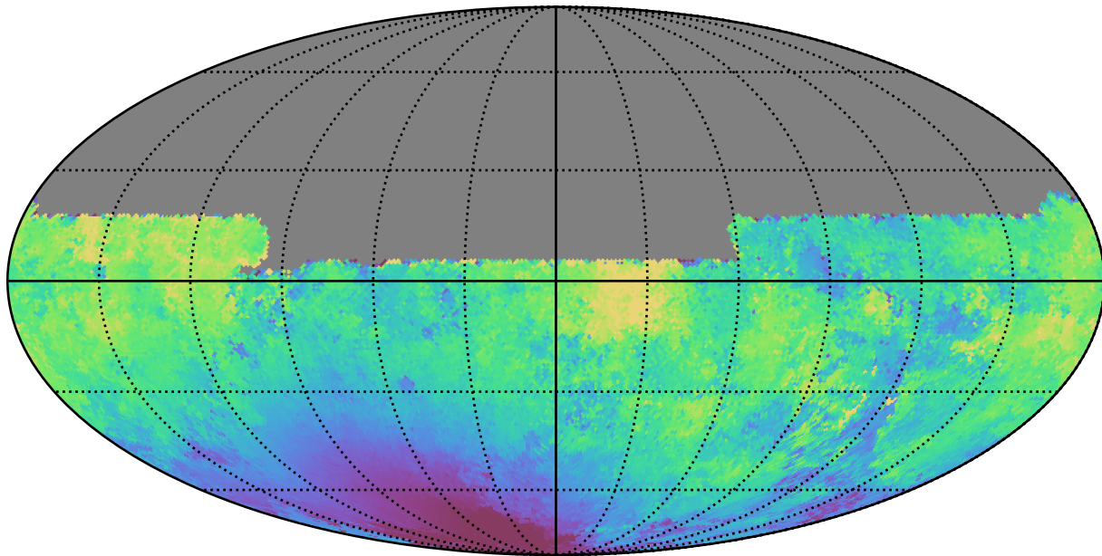
all_long_v3.4_10yrs All sky u band: Median moonDistance
