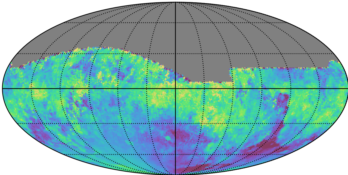
all_long_v3.4_10yrs All sky i band: Median moonDistance
