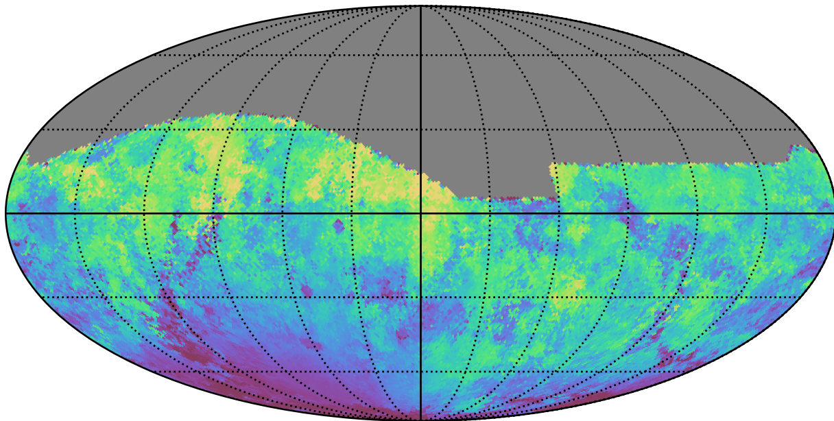
all_long_v3.4_10yrs All sky g band: Median moonDistance
