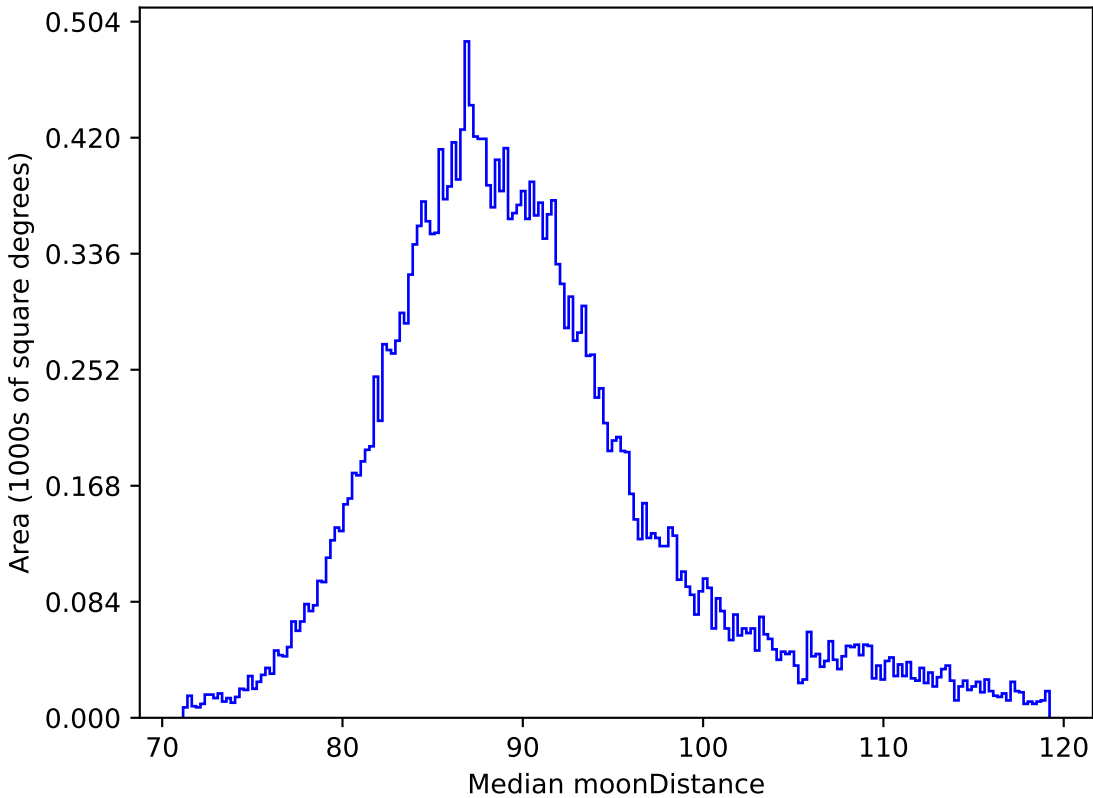
all_long_v3.4_10yrs All sky all bands: Median moonDistance
