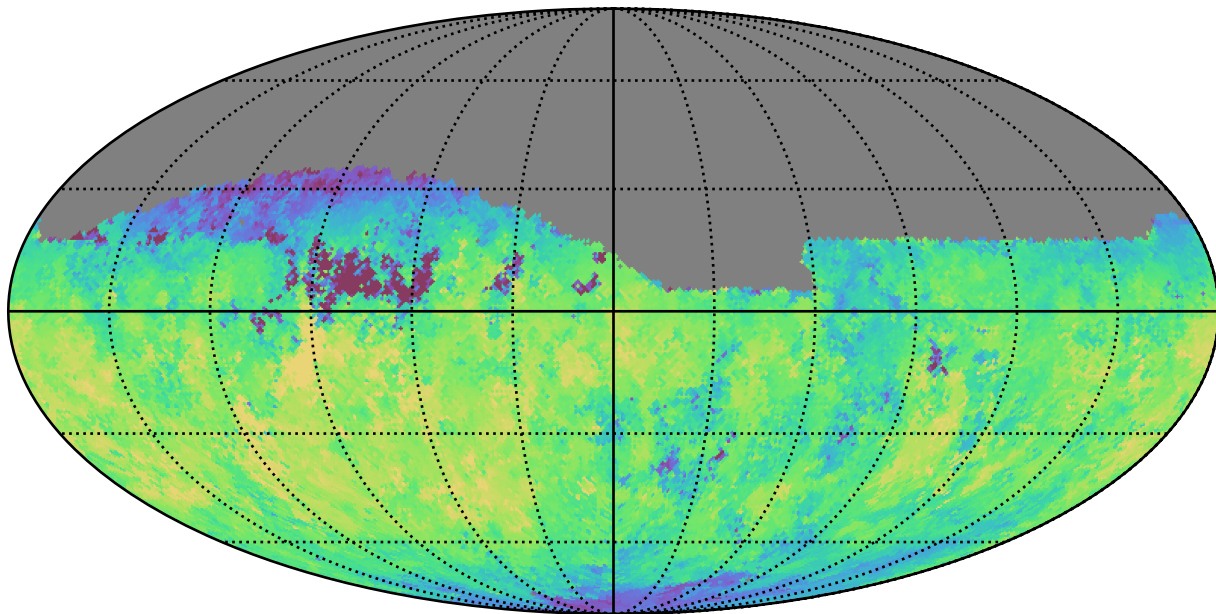
all_long_v3.4_10yrs Yr 1 z band: Median fiveSigmaDepth
