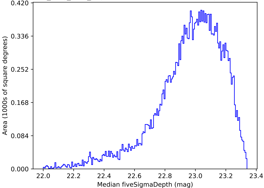
all_long_v3.4_10yrs Yr 1 z band: Median fiveSigmaDepth
