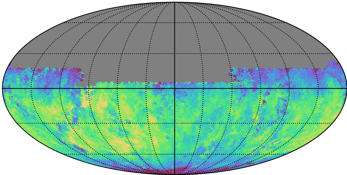
all_long_v3.4_10yrs Yr 1 y band: Median fiveSigmaDepth
