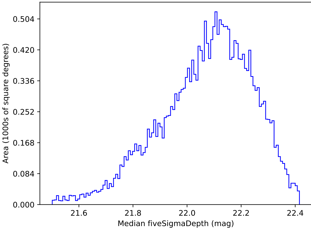
all_long_v3.4_10yrs Yr 1 y band: Median fiveSigmaDepth
