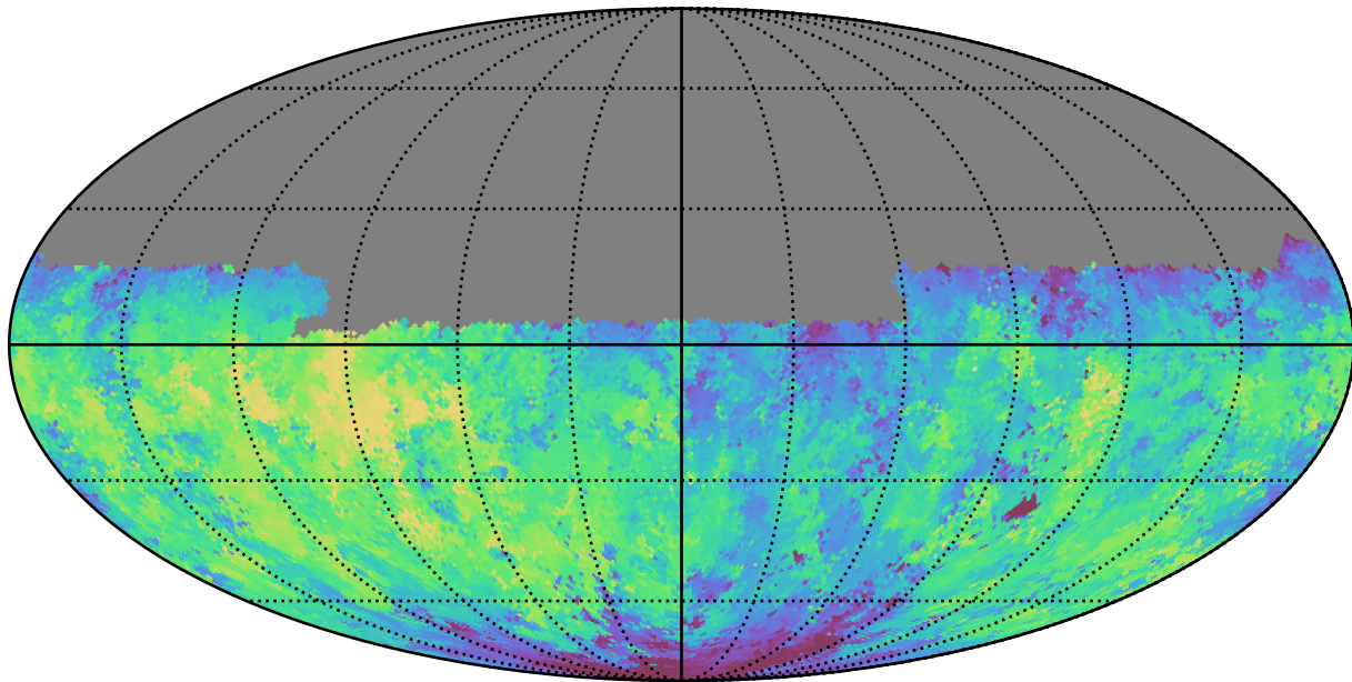
all_long_v3.4_10yrs Yr 1 u band: Median fiveSigmaDepth
