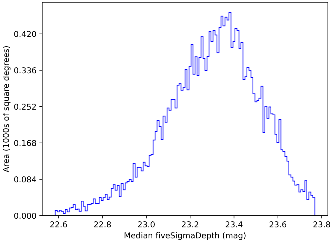
all_long_v3.4_10yrs Yr 1 u band: Median fiveSigmaDepth
