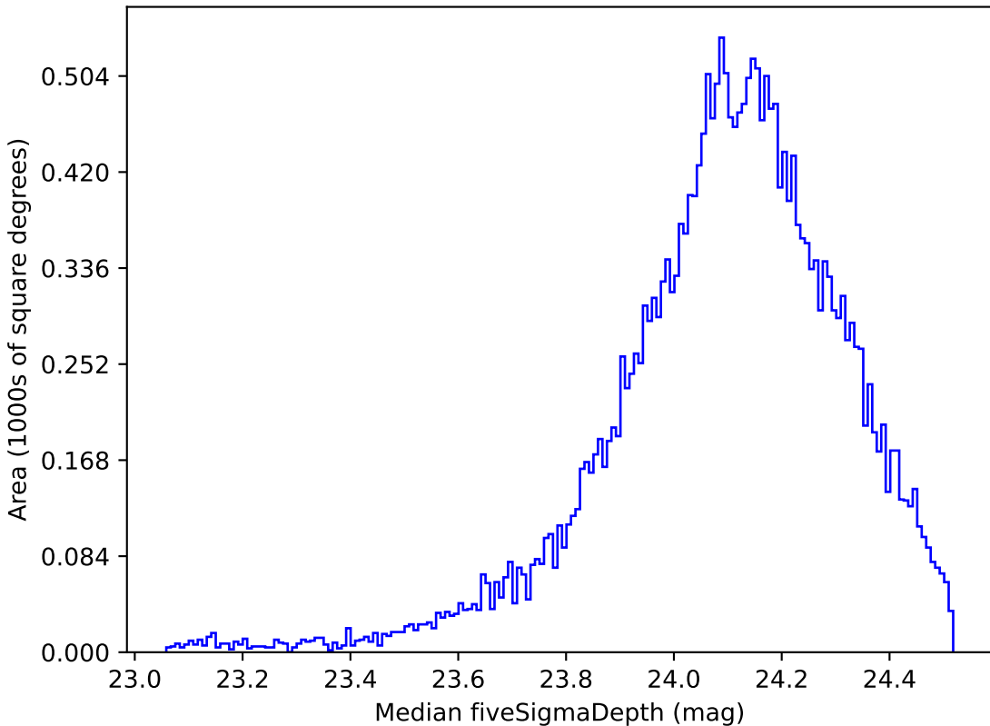
all_long_v3.4_10yrs Yr 1 r band: Median fiveSigmaDepth
