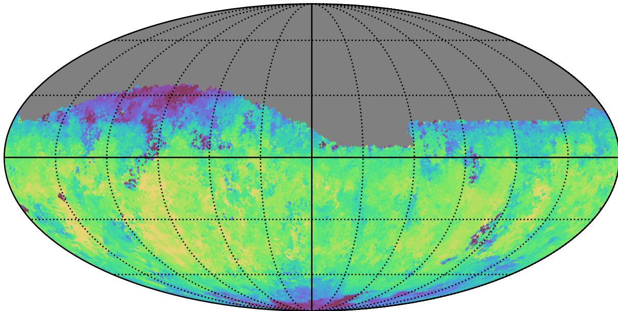
all_long_v3.4_10yrs Yr 1 i band: Median fiveSigmaDepth
